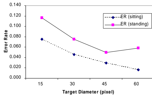
Figure 4. Mean error rates for each posture by target diameter when using a trackball.
